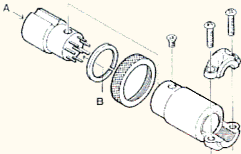
Plug assembly
